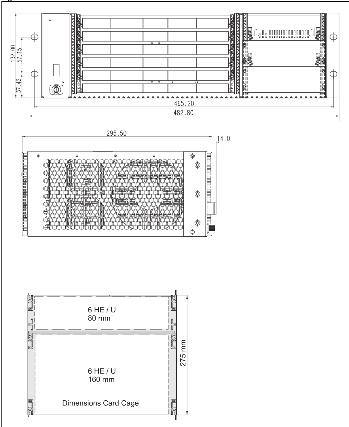
Figure 6: Maße
